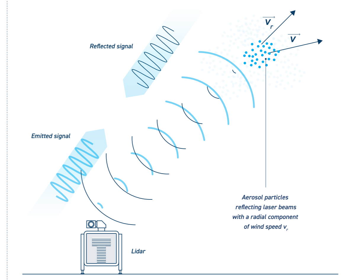
Lidar measurement
