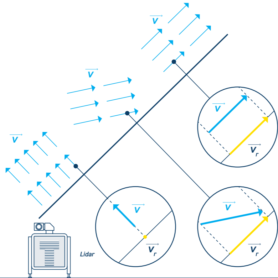
Detection of the radial component of wind speed by lidar
