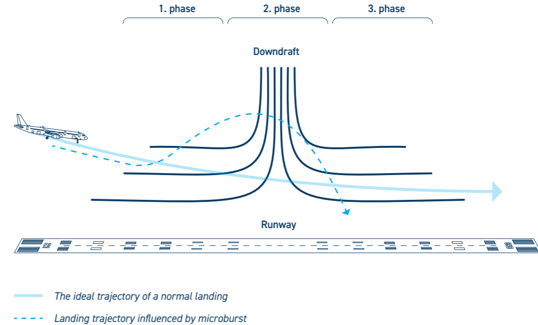
Aircraft flight through a microburst
